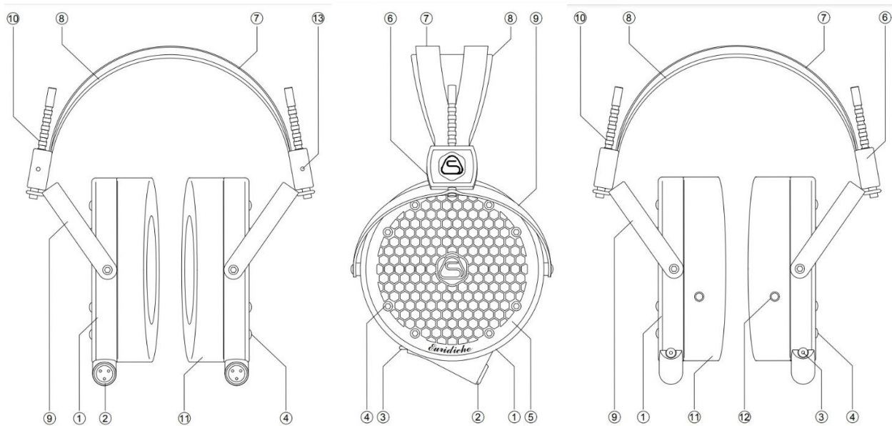
Figure 1. Headphones: front, side and rear views
